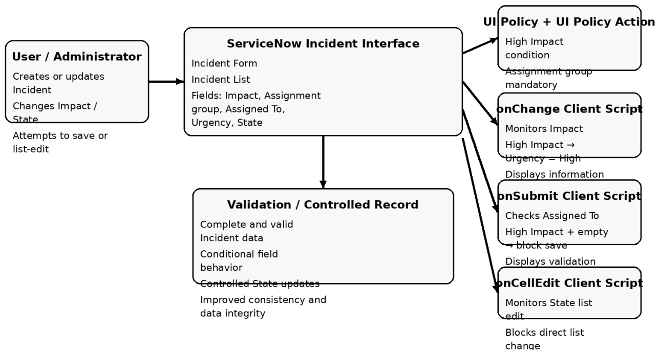
Figure 1: Solution architecture and data flow for Implement Client Script & UI Policy (Incident)
